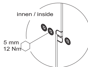
DETAIL X
