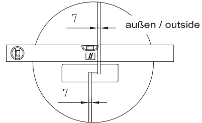
DETAIL X
